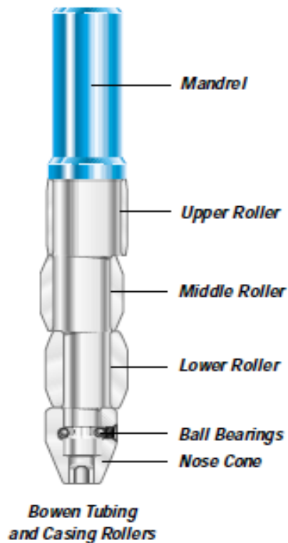
Gambar : Casing Rollers
